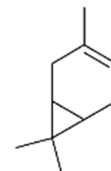
3-caren
