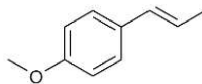
anethol
